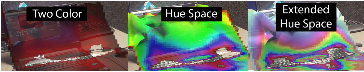
Figure 3: This image was taken via screen capture on the HoloLens 2 and depicts the three visualization modes available for use in the prototype extended perception system across a temperature range of 27 to 38 degrees Celsius.
