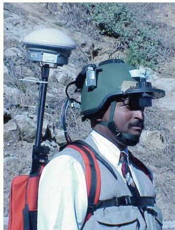
10 HRL Laboratories prototype person-portable mobile augmented reality system with GPS, inertial, and magnetic sensors.
