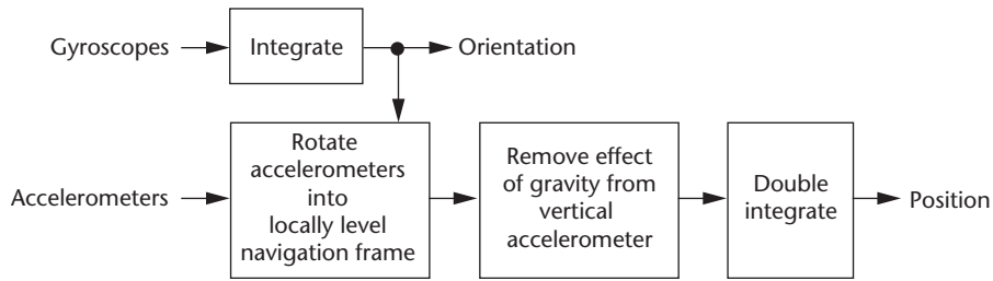
2 Basic strap-down inertial navigation algorithm.
