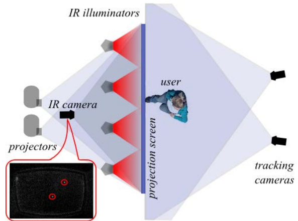
Figure 2: Sketch of stereoscopic multi-touch surface setup.
